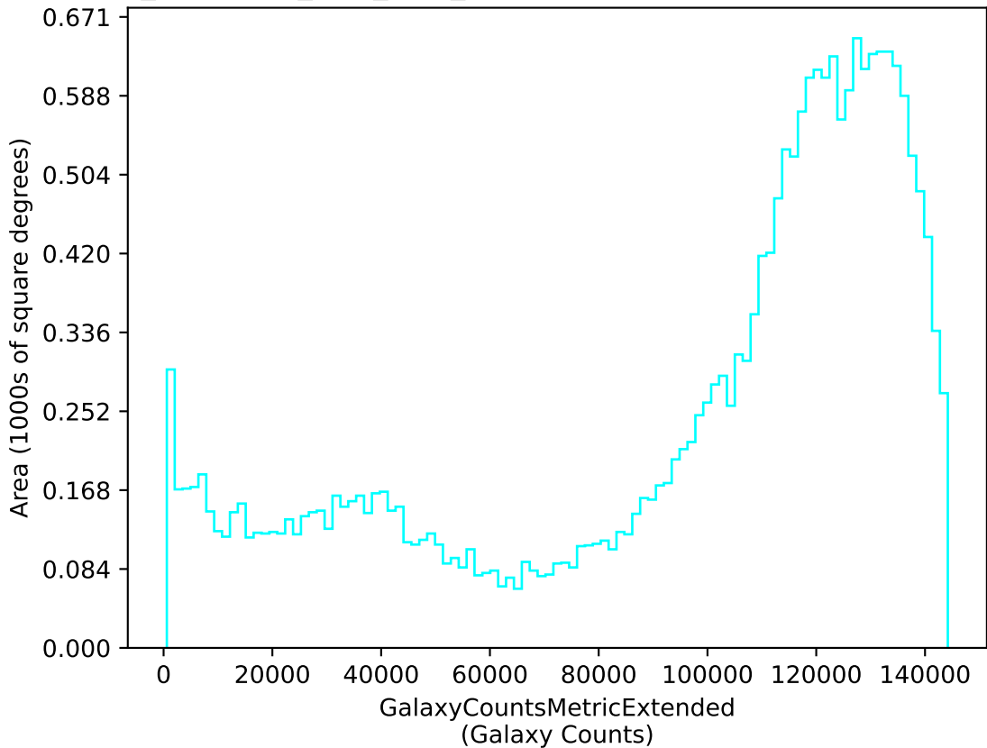
too_combined_s0.5_v3.4_10yrs u: GalaxyCountsMetricExtended
