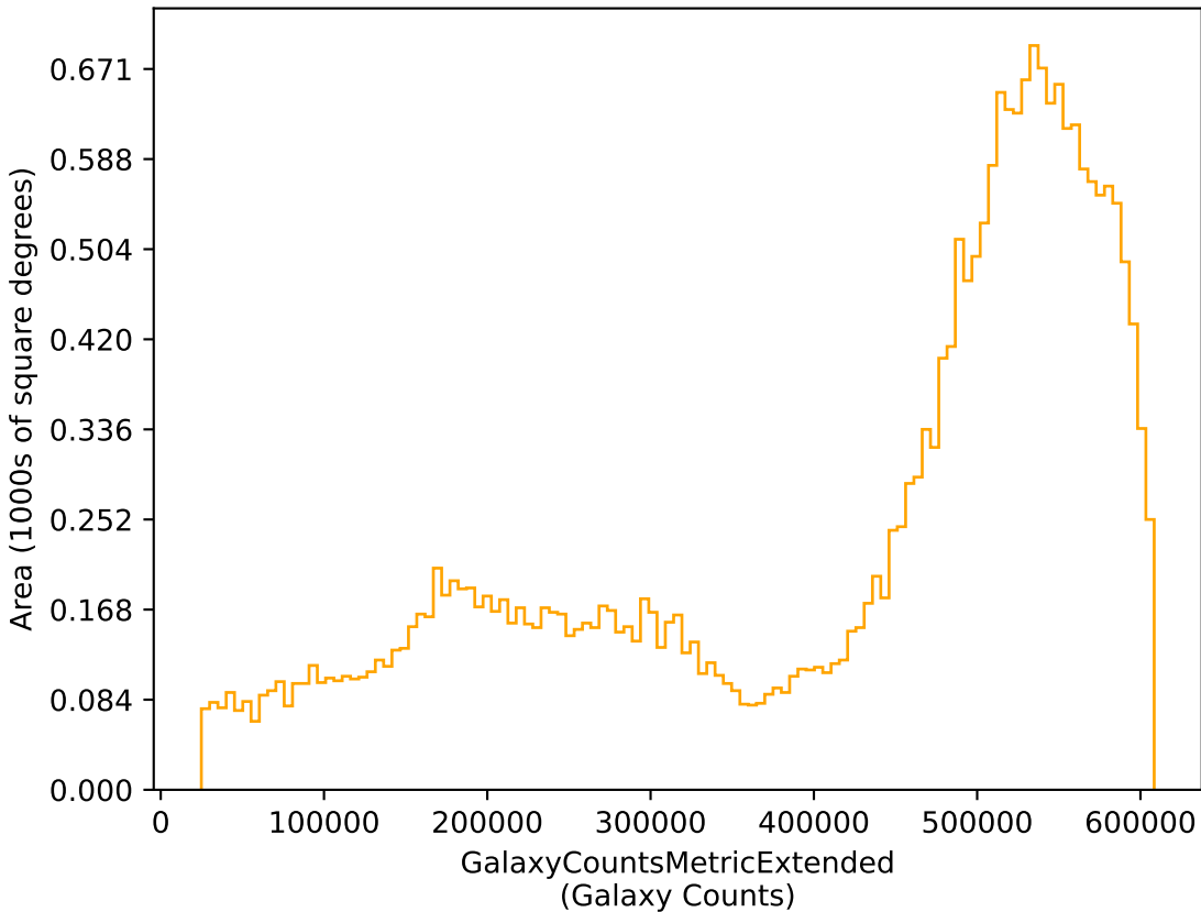
too_combined_s0.5_v3.4_10yrs r: GalaxyCountsMetricExtended
