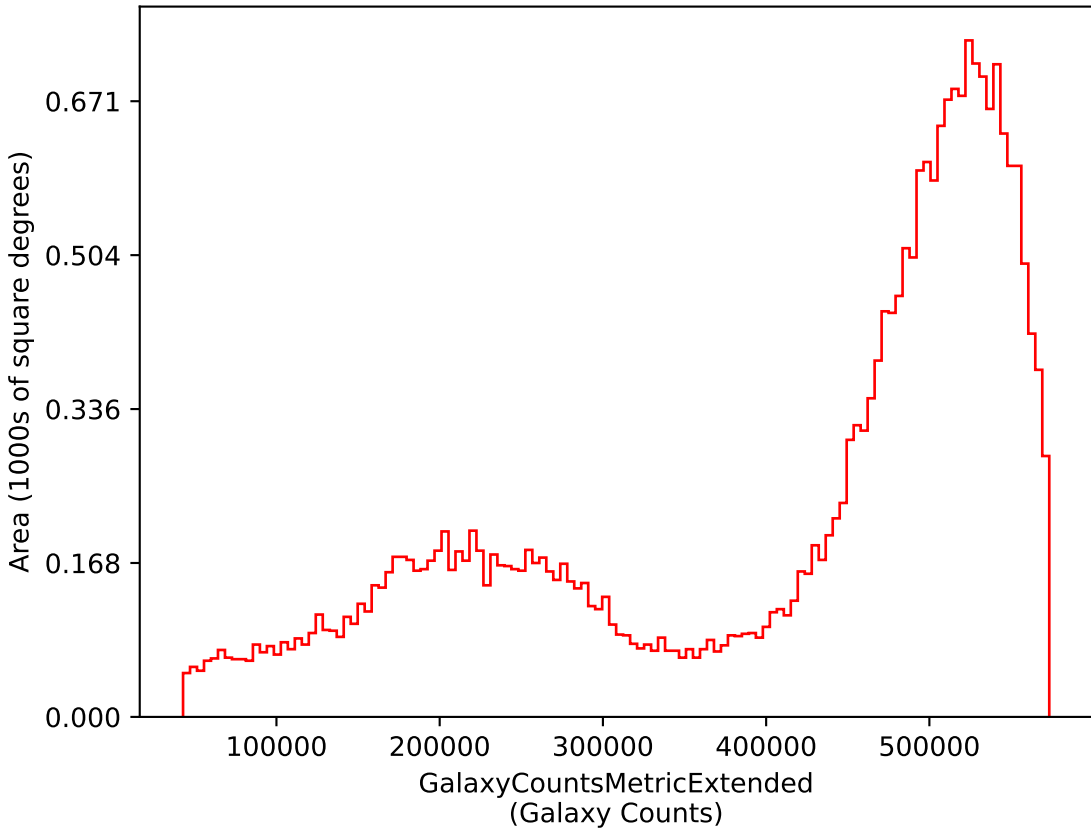
too_combined_s0.5_v3.4_10yrs i: GalaxyCountsMetricExtended
