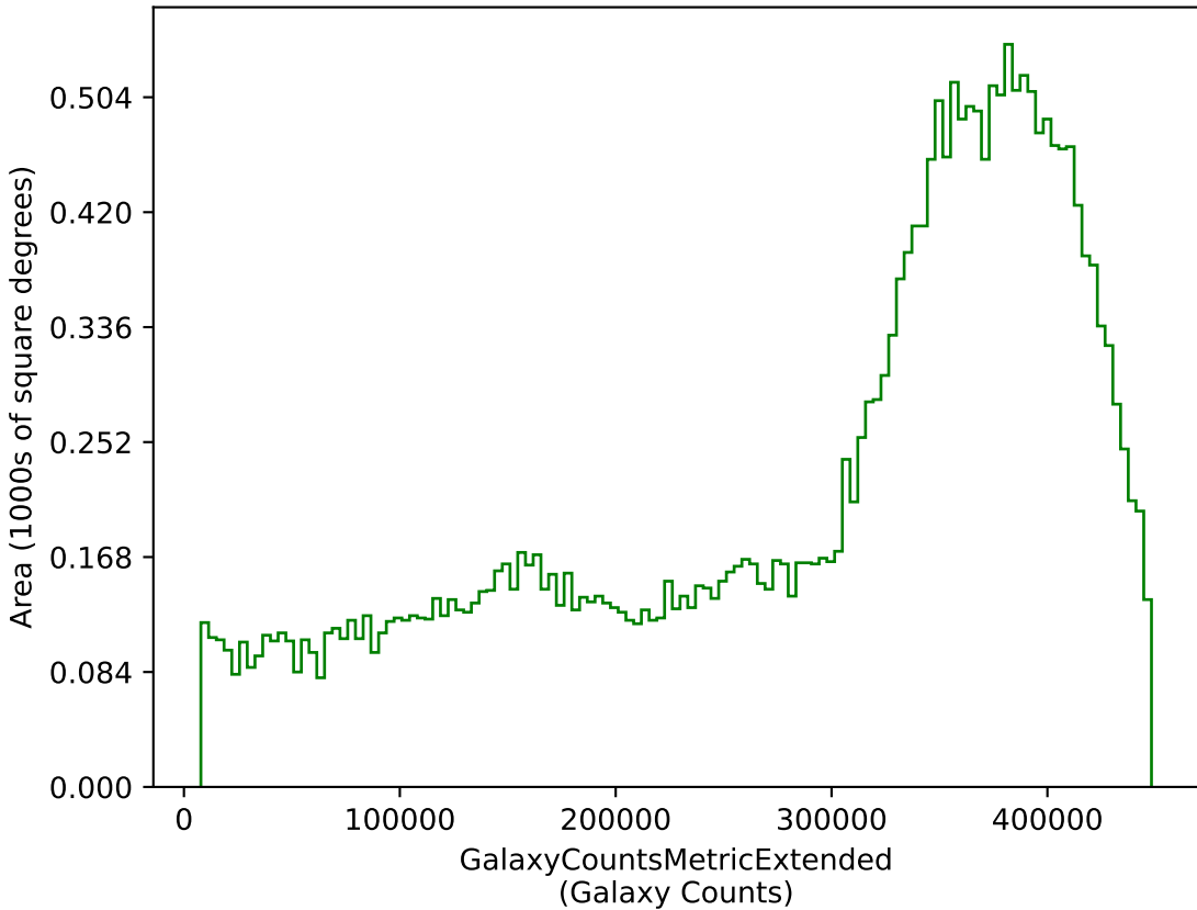
too_combined_s0.5_v3.4_10yrs g: GalaxyCountsMetricExtended
