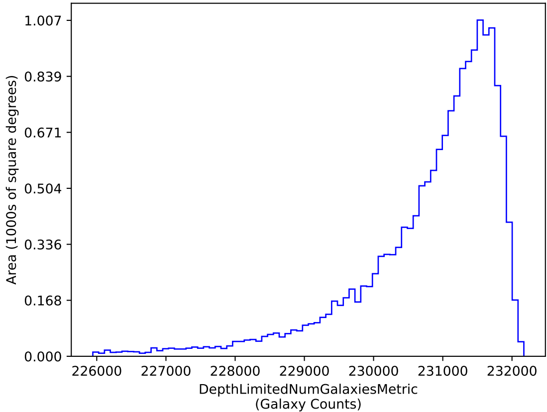
too_combined_s0.5_v3.4_10yrs i band galaxies non-DD: DepthLimitedNumGalaxiesMetric
