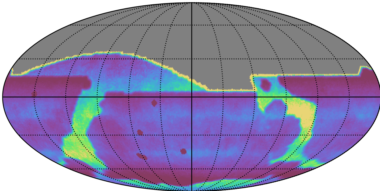
too_combined_s0.5_v3.4_10yrs : DCRprecision
