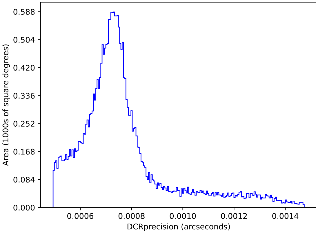
too_combined_s0.5_v3.4_10yrs : DCRprecision
