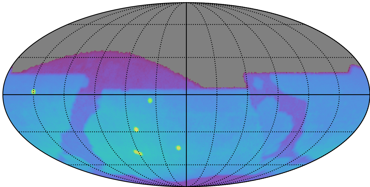
too_combined_s0.5_v3.4_10yrs : Brown Dwarf, L7
