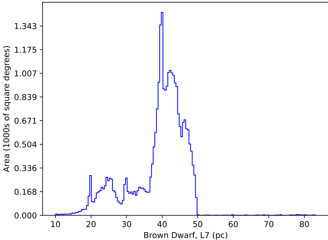
too_combined_s0.5_v3.4_10yrs : Brown Dwarf, L7
