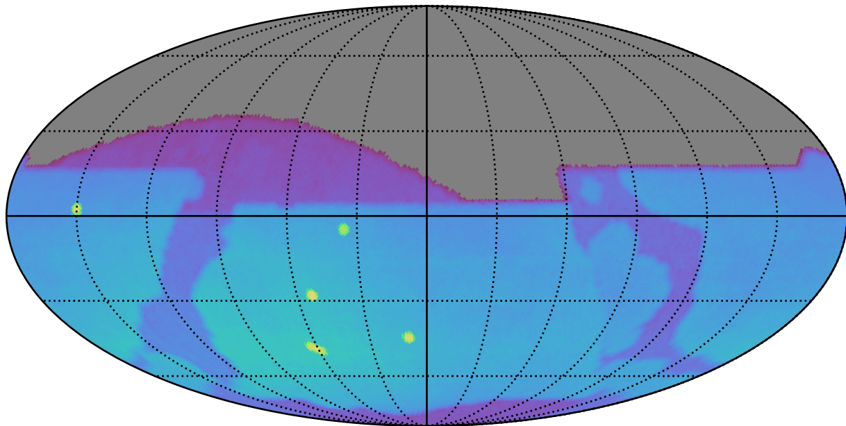
too_combined_s0.5_v3.4_10yrs : Brown Dwarf, L4
