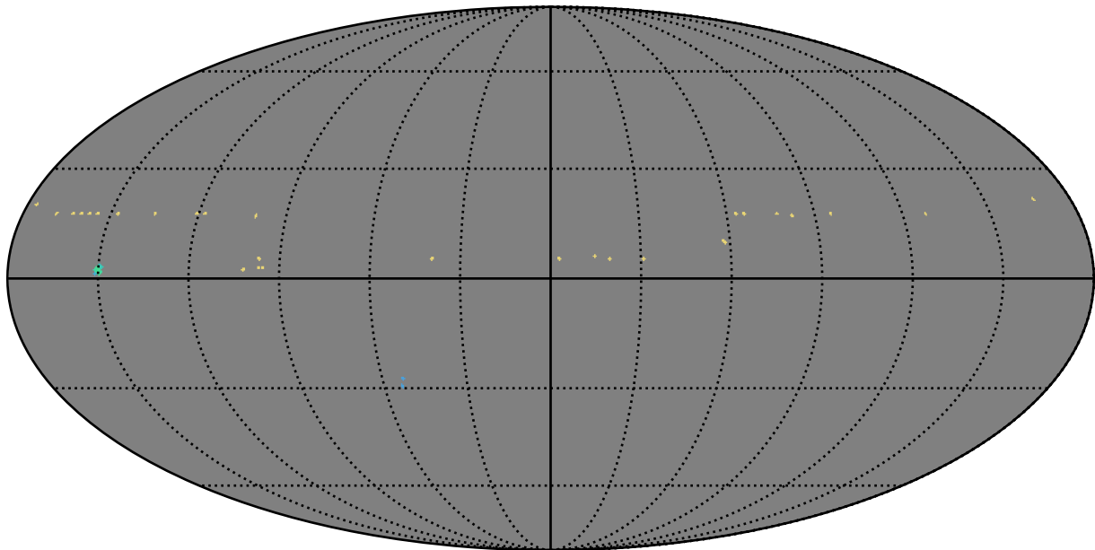
too_combined_s0.5_v3.4_10yrs y band: AGN_TimeLag_5_days
