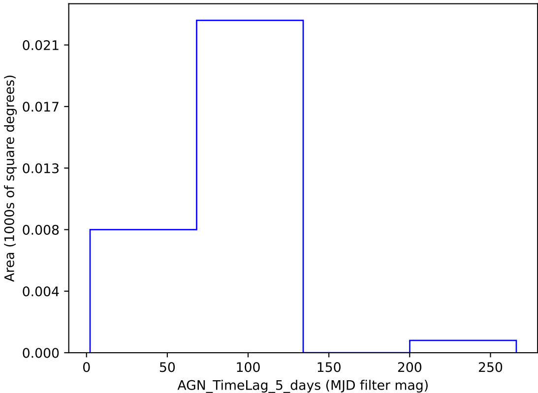
too_combined_s0.5_v3.4_10yrs y band: AGN_TimeLag_5_days
