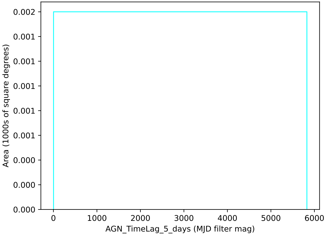
too_combined_s0.5_v3.4_10yrs u band: AGN_TimeLag_5_days
