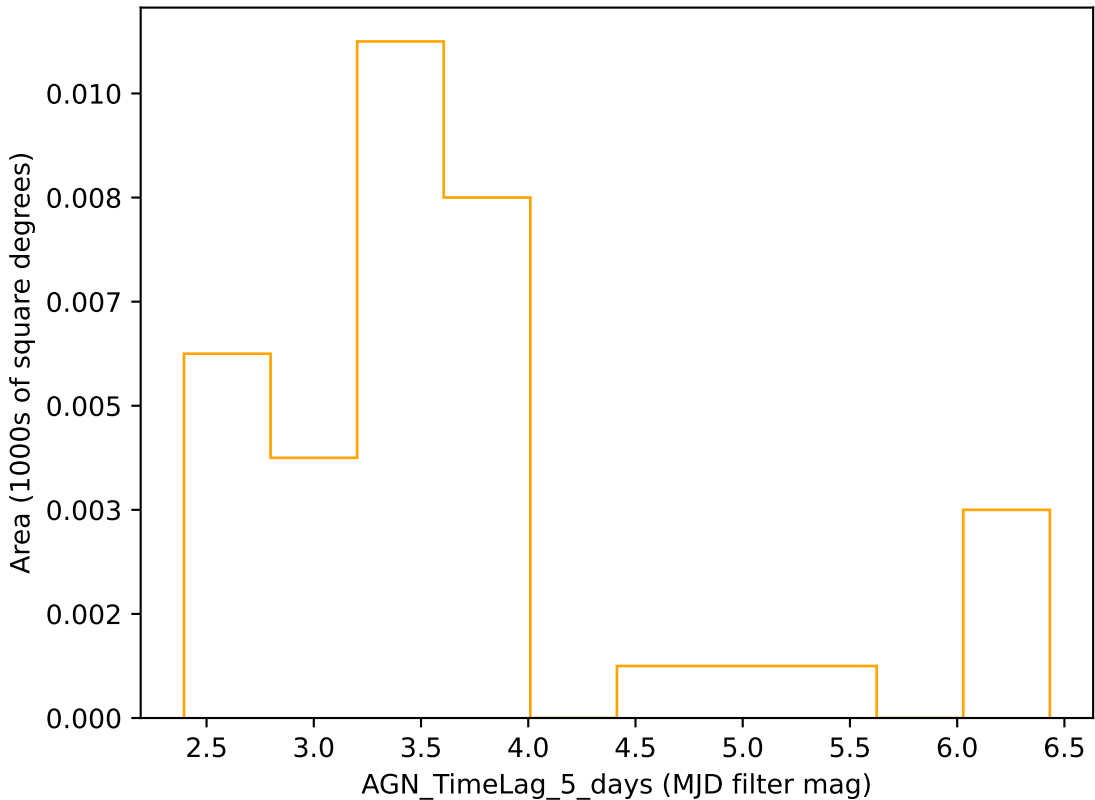
too_combined_s0.5_v3.4_10yrs r band: AGN_TimeLag_5_days
