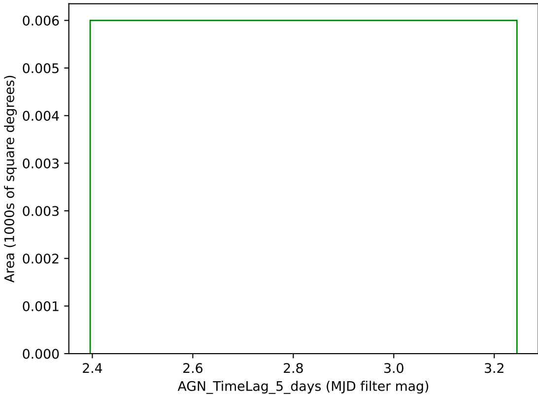
too_combined_s0.5_v3.4_10yrs g band: AGN_TimeLag_5_days
