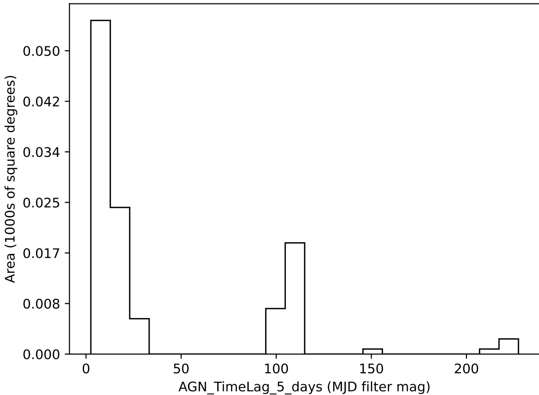
too_combined_s0.5_v3.4_10yrs all bands: AGN_TimeLag_5_days
