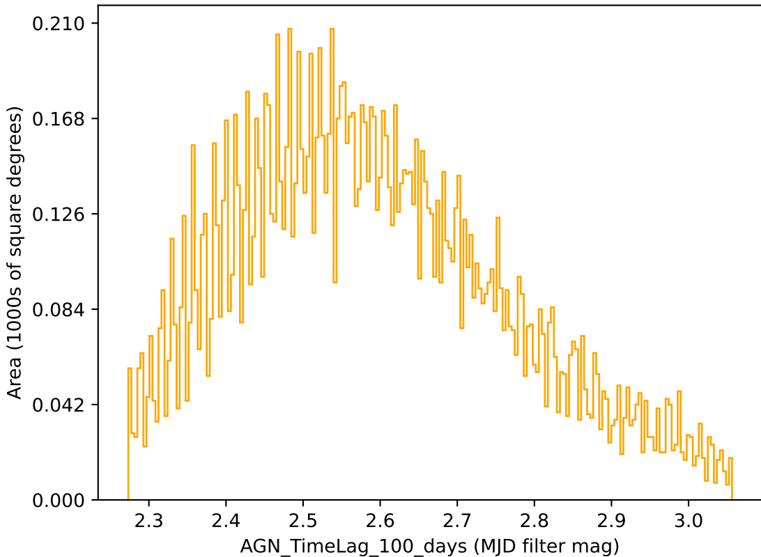
too_combined_s0.5_v3.4_10yrs r band: AGN_TimeLag_100_days
