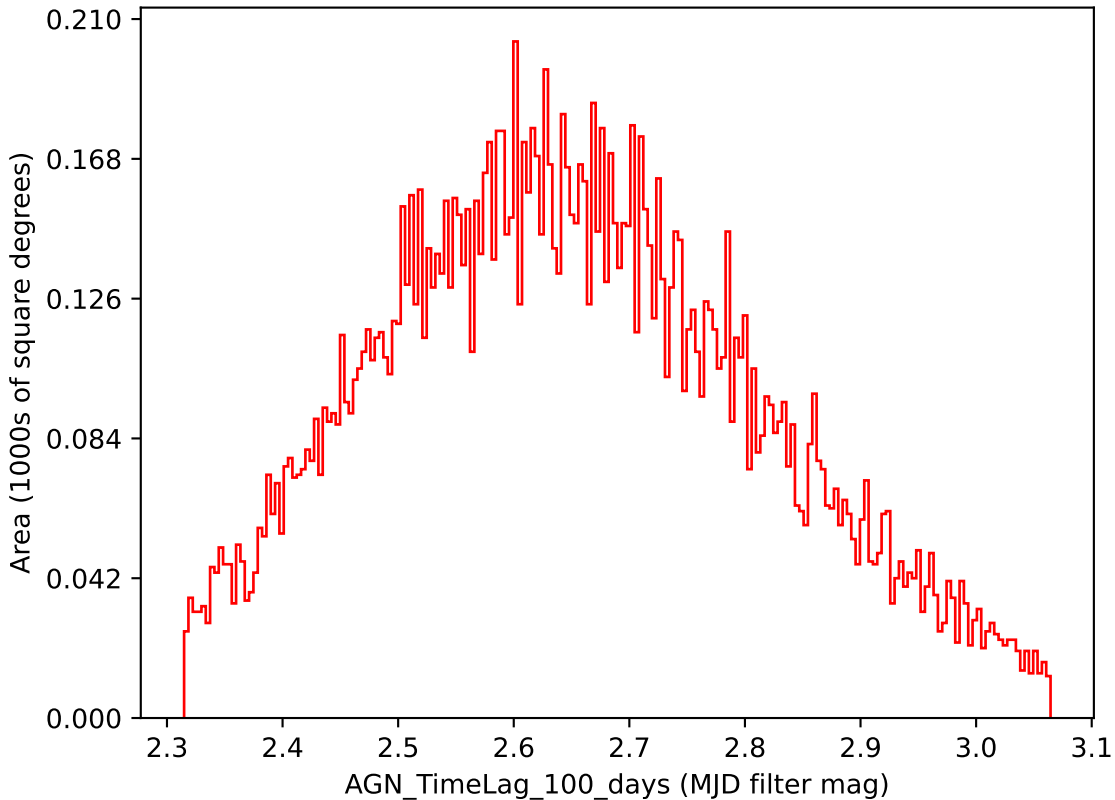
too_combined_s0.5_v3.4_10yrs i band: AGN_TimeLag_100_days
