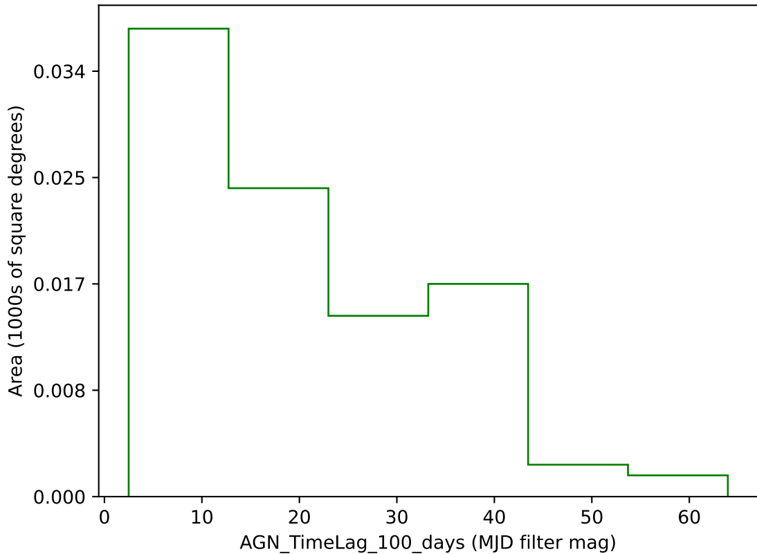
too_combined_s0.5_v3.4_10yrs g band: AGN_TimeLag_100_days
