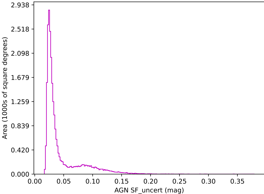
too_combined_s0.5_v3.4_10yrs z band: AGN SF_uncert
