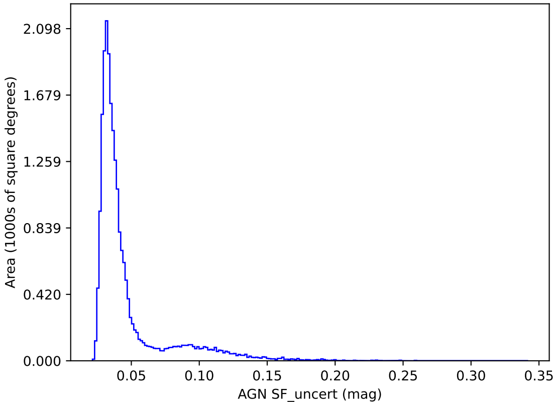
too_combined_s0.5_v3.4_10yrs y band: AGN SF_uncert
