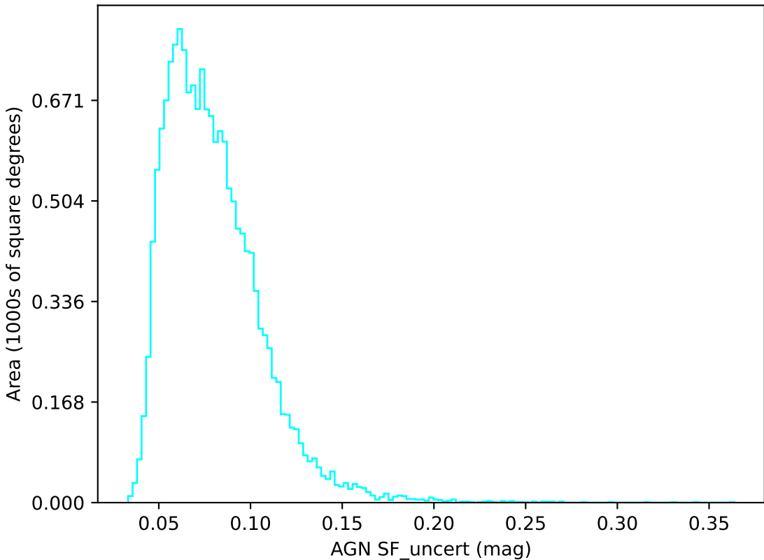
too_combined_s0.5_v3.4_10yrs u band: AGN SF_uncert
