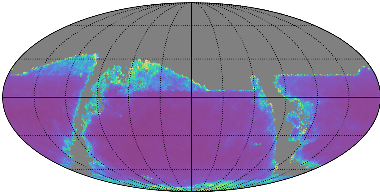
too_combined_s0.5_v3.4_10yrs i band: AGN SF_uncert
