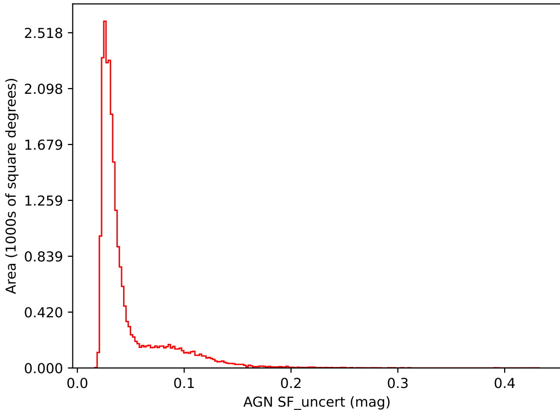
too_combined_s0.5_v3.4_10yrs i band: AGN SF_uncert
