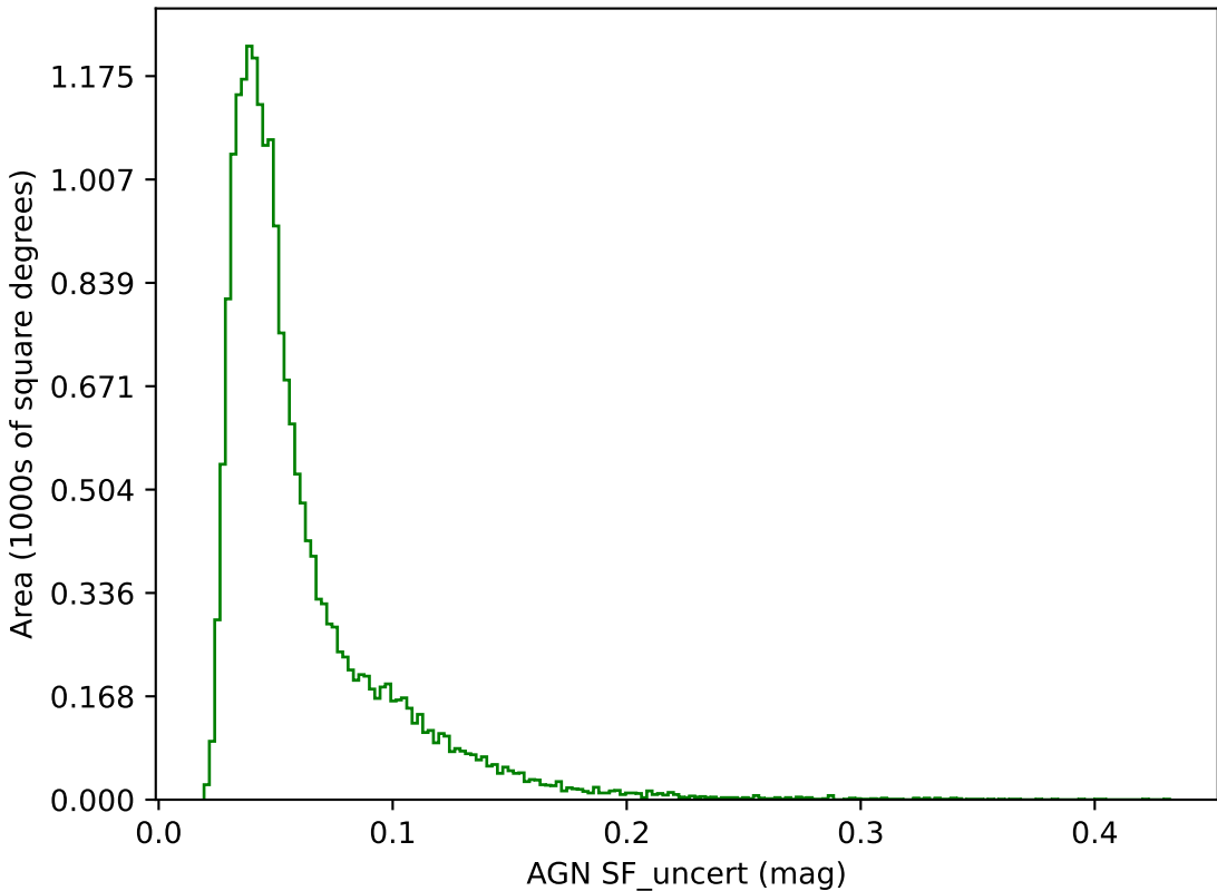
too_combined_s0.5_v3.4_10yrs g band: AGN SF_uncert
