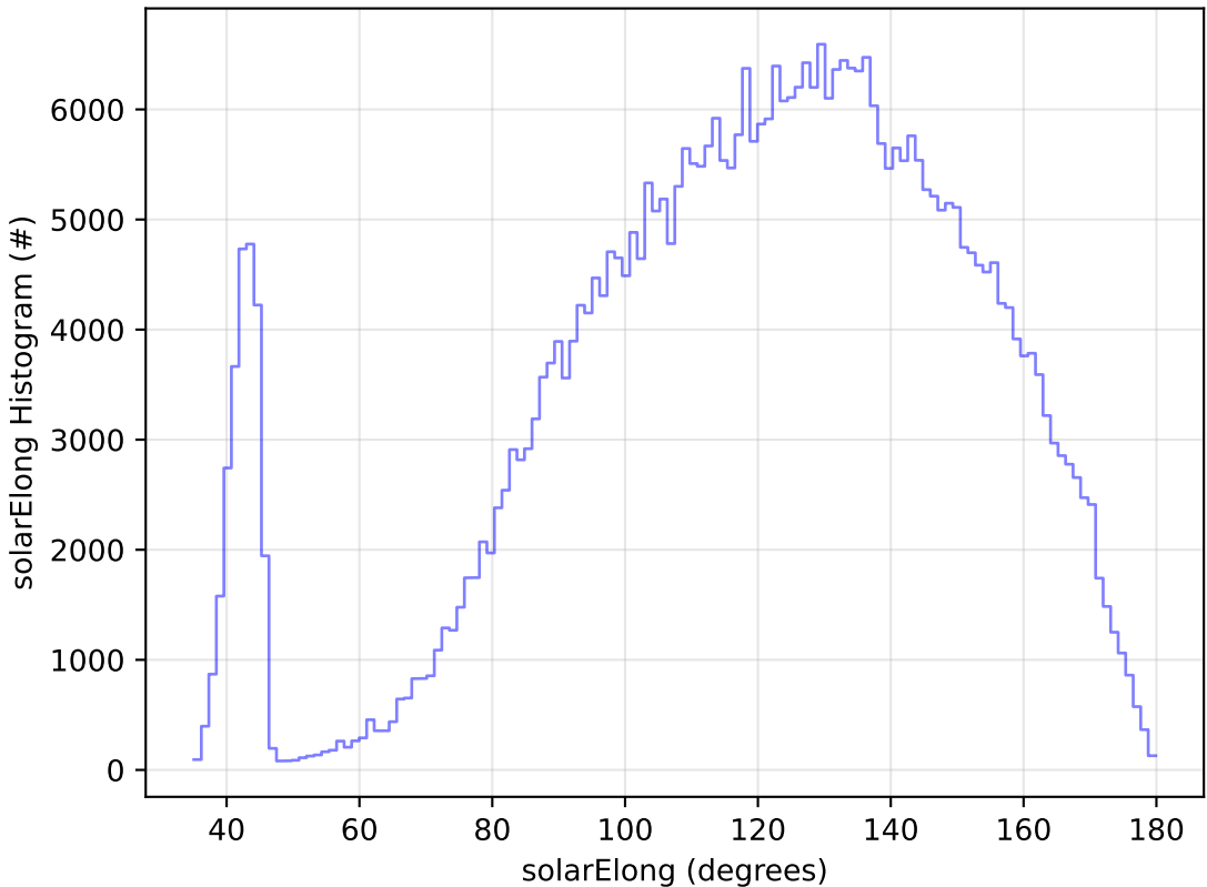
too_combined_s0.5_v3.4_10yrs WFD z band: solarElong Histogram
