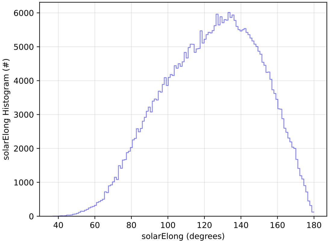
too_combined_s0.5_v3.4_10yrs WFD y band: solarElong Histogram
