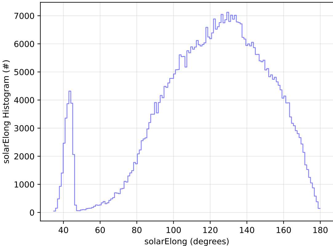
too_combined_s0.5_v3.4_10yrs WFD i band: solarElong Histogram
