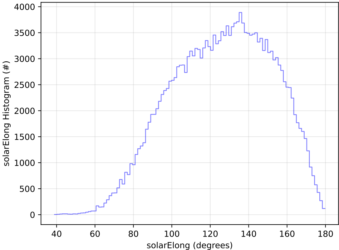
too_combined_s0.5_v3.4_10yrs WFD g band: solarElong Histogram
