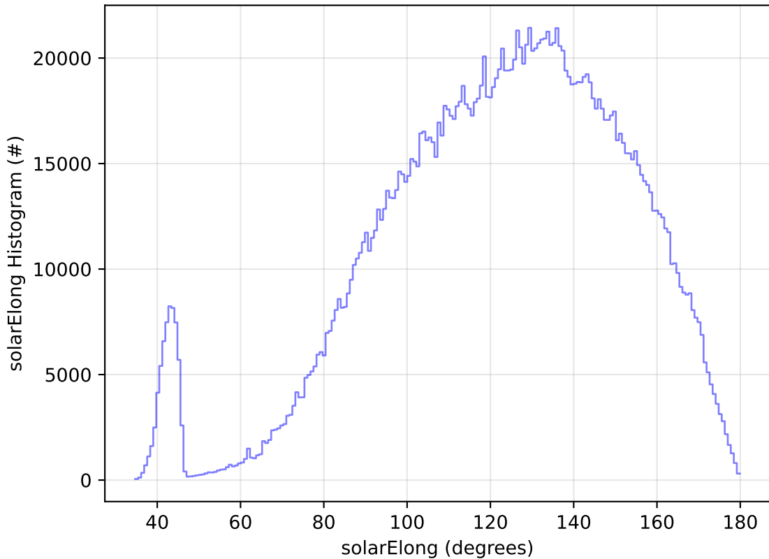
too_combined_s0.5_v3.4_10yrs WFD all bands: solarElong Histogram
