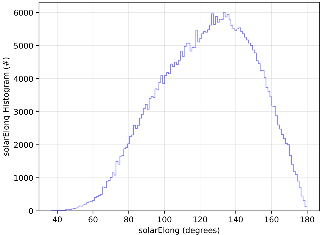
too_combined_s0.5_v3.4_10yrs All sky y band: solarElong Histogram
