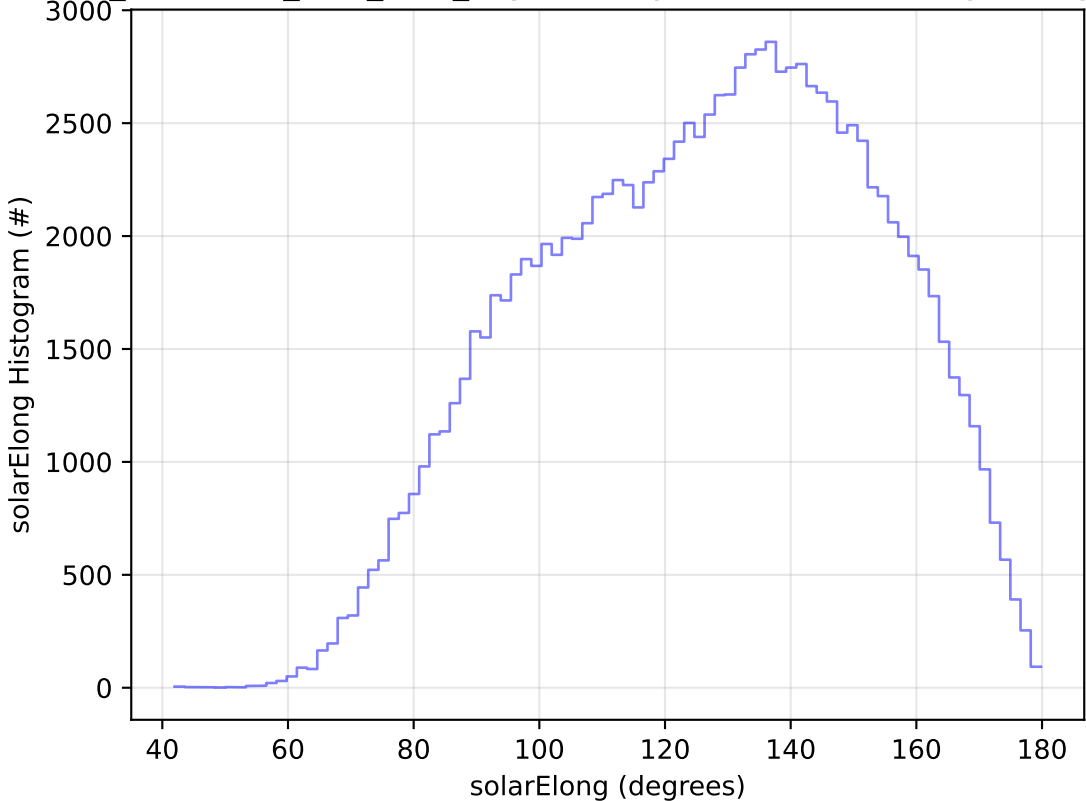
too_combined_s0.5_v3.4_10yrs All sky u band: solarElong Histogram
