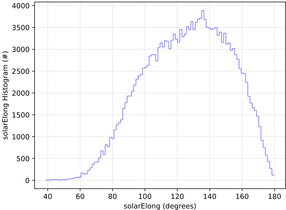
too_combined_s0.5_v3.4_10yrs All sky g band: solarElong Histogram
