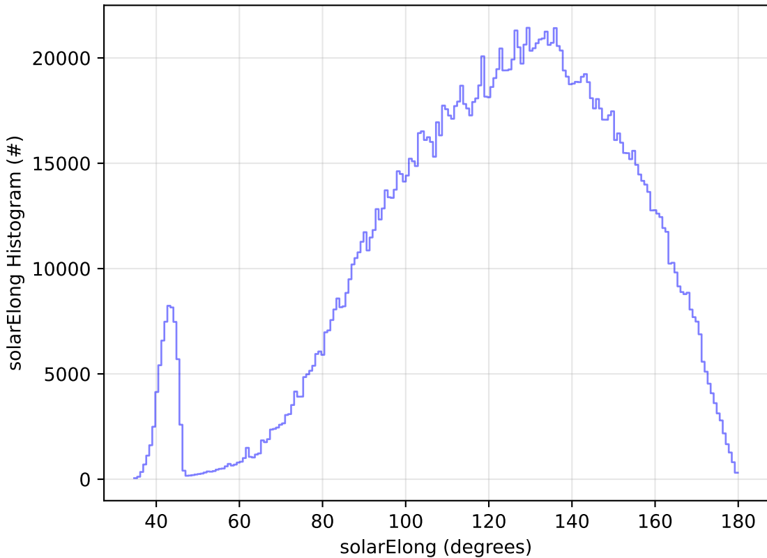
too_combined_s0.5_v3.4_10yrs All sky all bands: solarElong Histogram
