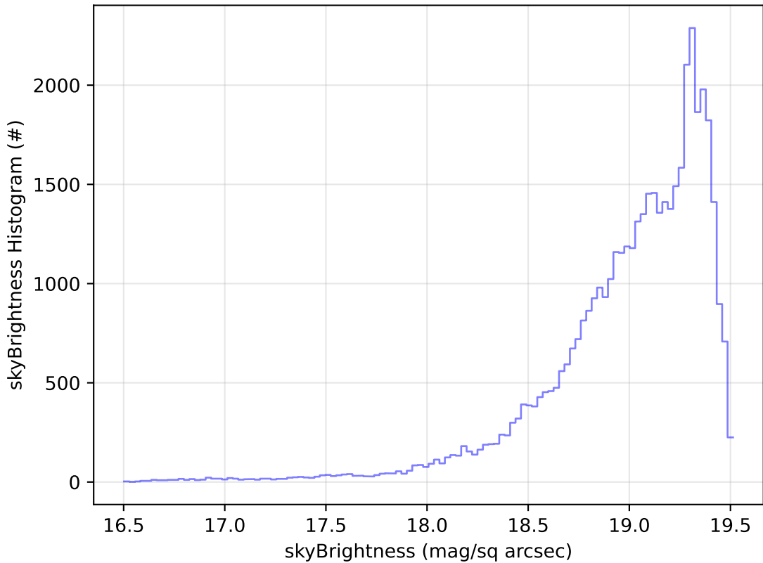
too_combined_s0.5_v3.4_10yrs Yr 1 z band: skyBrightness Histogram
