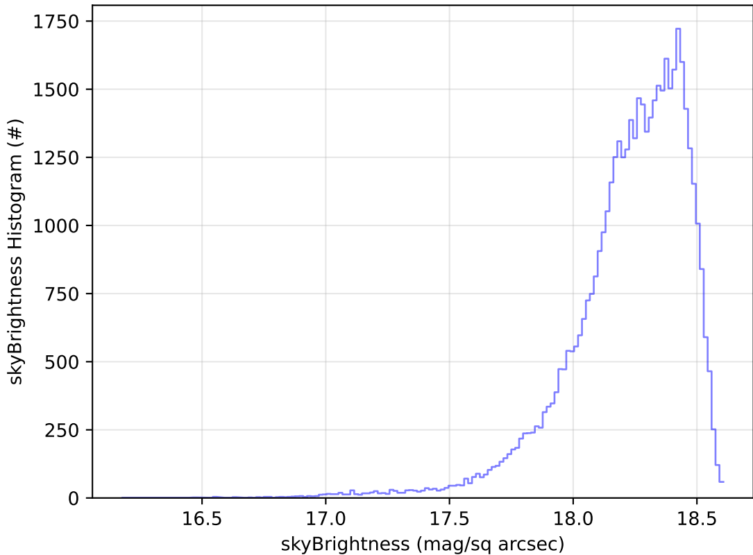
too_combined_s0.5_v3.4_10yrs Yr 1 y band: skyBrightness Histogram
