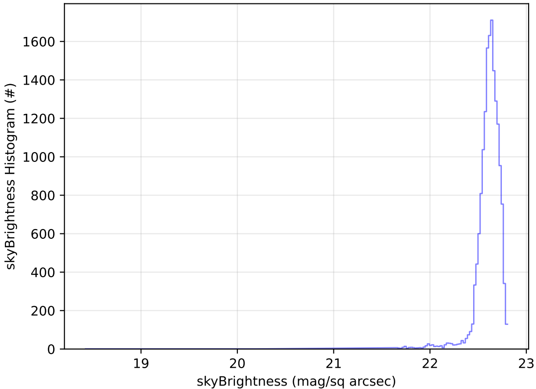
too_combined_s0.5_v3.4_10yrs Yr 1 u band: skyBrightness Histogram
