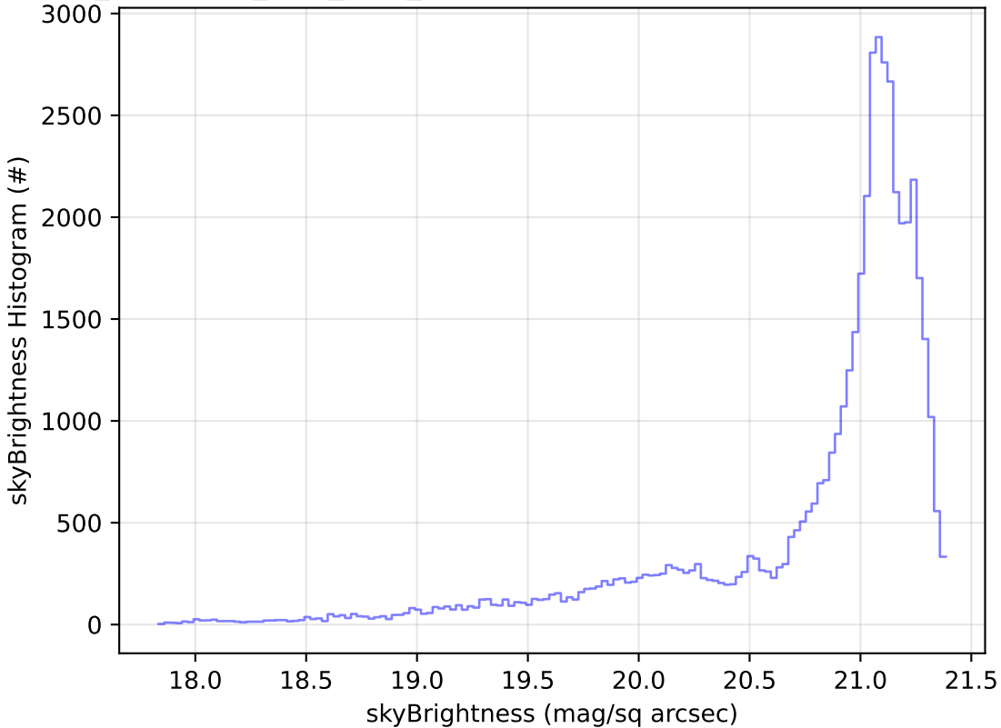
too_combined_s0.5_v3.4_10yrs Yr 1 r band: skyBrightness Histogram
