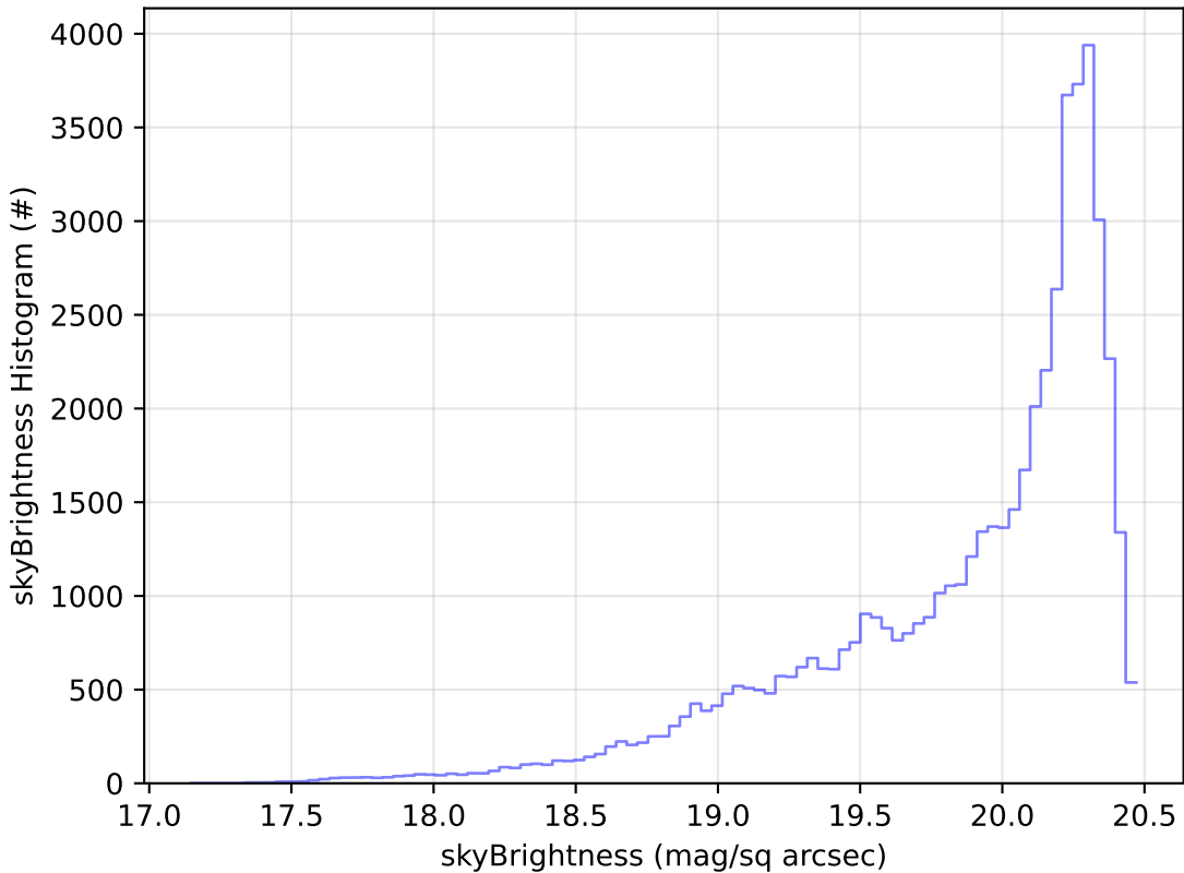
too_combined_s0.5_v3.4_10yrs Yr 1 i band: skyBrightness Histogram
