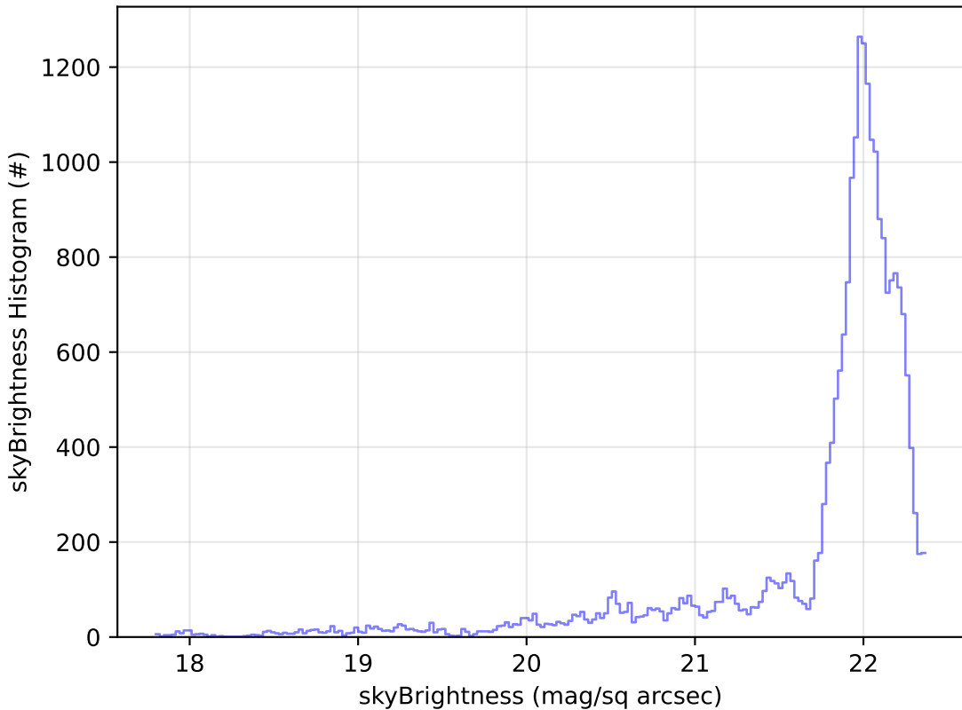
too_combined_s0.5_v3.4_10yrs Yr 1 g band: skyBrightness Histogram
