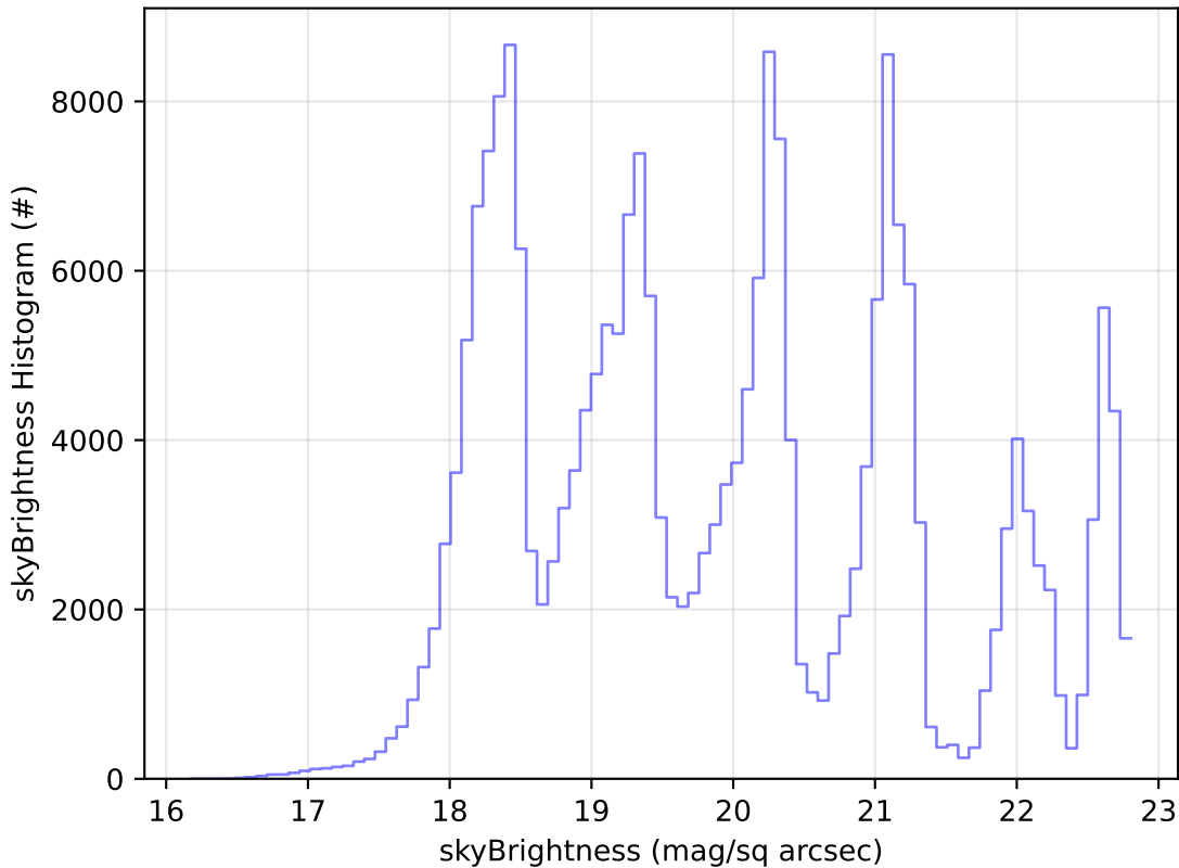
too_combined_s0.5_v3.4_10yrs Yr 1 all bands: skyBrightness Histogram
