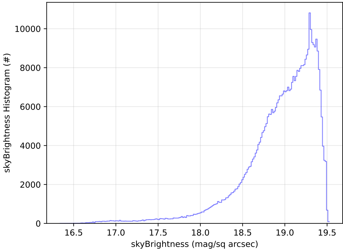
too_combined_s0.5_v3.4_10yrs WFD z band: skyBrightness Histogram
