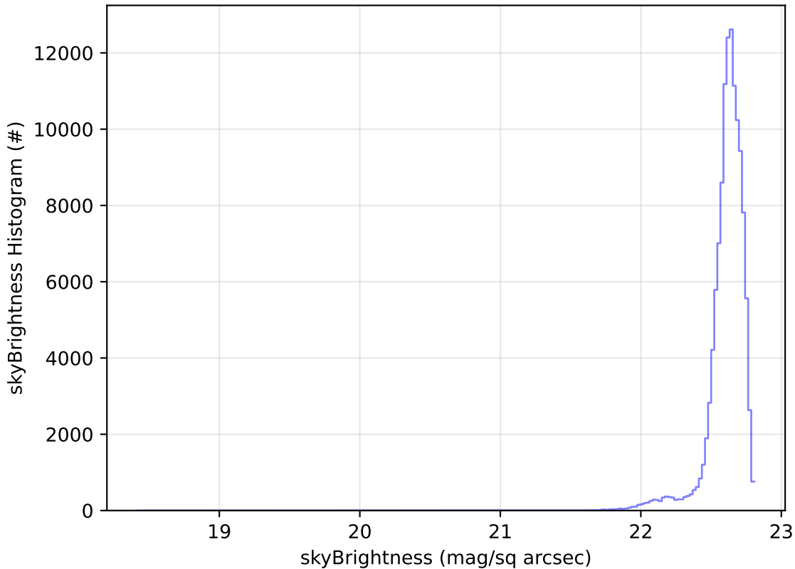
too_combined_s0.5_v3.4_10yrs WFD u band: skyBrightness Histogram
