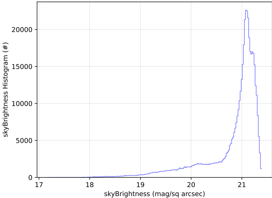
too_combined_s0.5_v3.4_10yrs WFD r band: skyBrightness Histogram
