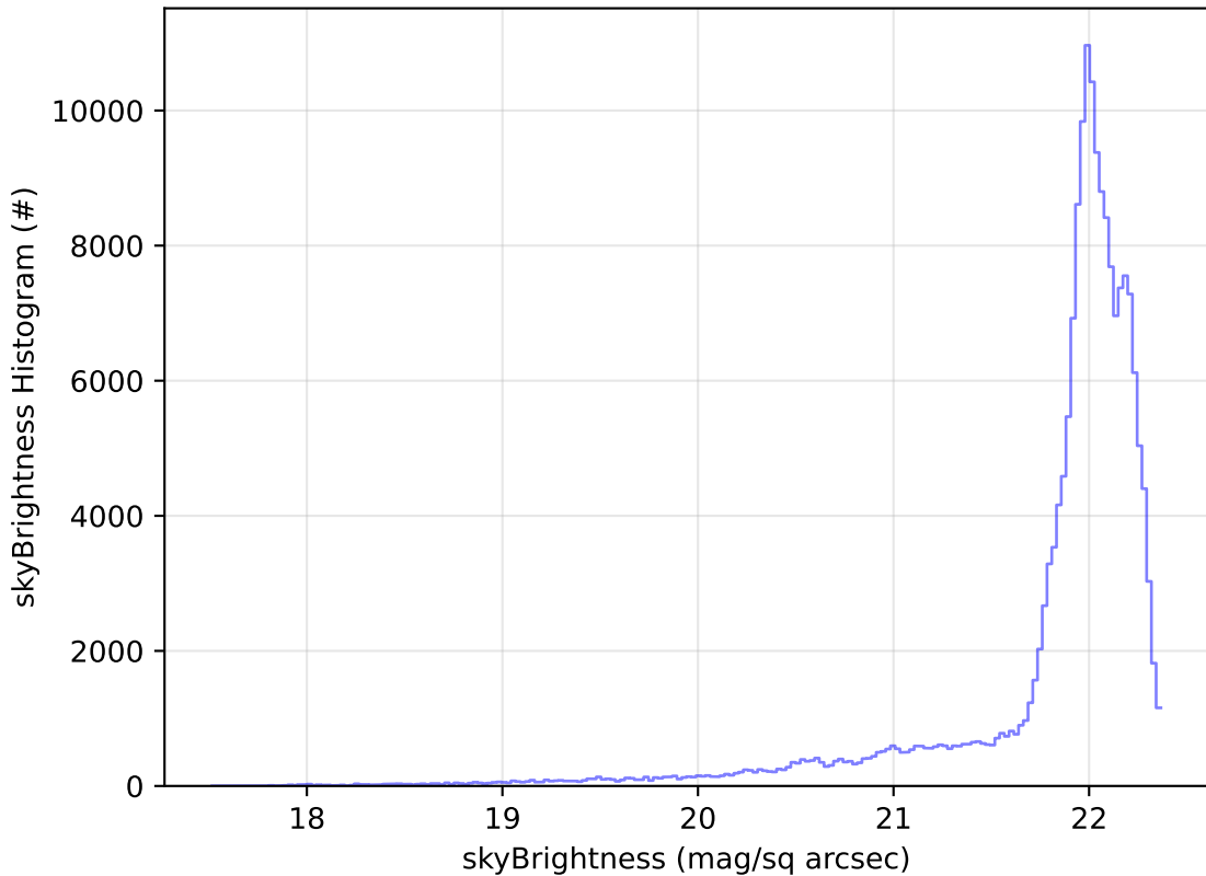
too_combined_s0.5_v3.4_10yrs WFD g band: skyBrightness Histogram
