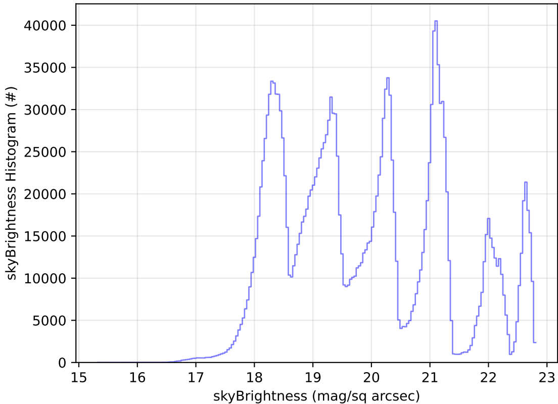
too_combined_s0.5_v3.4_10yrs WFD all bands: skyBrightness Histogram
