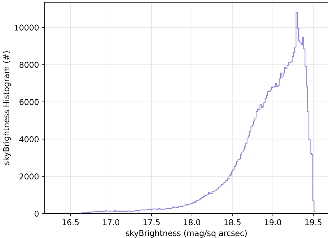
too_combined_s0.5_v3.4_10yrs All sky z band: skyBrightness Histogram
