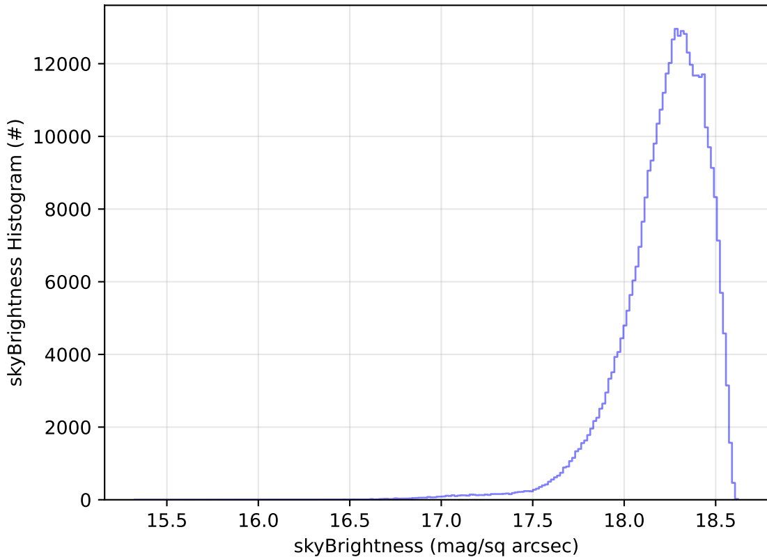
too_combined_s0.5_v3.4_10yrs All sky y band: skyBrightness Histogram
