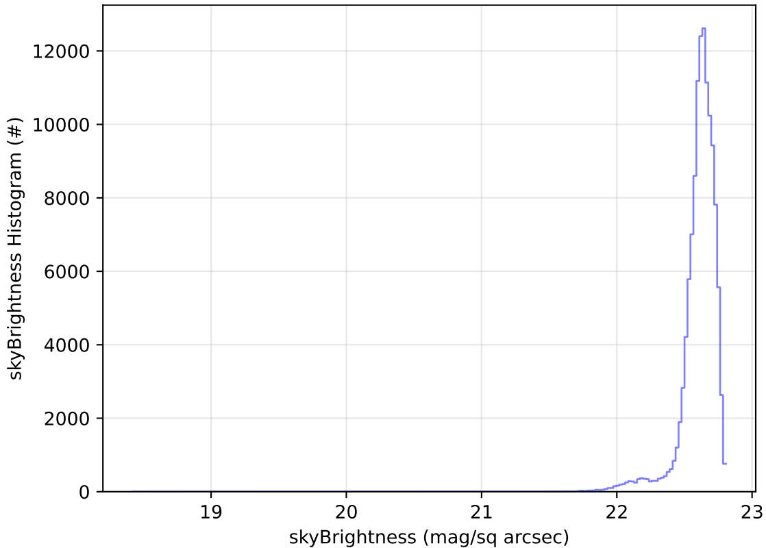
too_combined_s0.5_v3.4_10yrs All sky u band: skyBrightness Histogram
