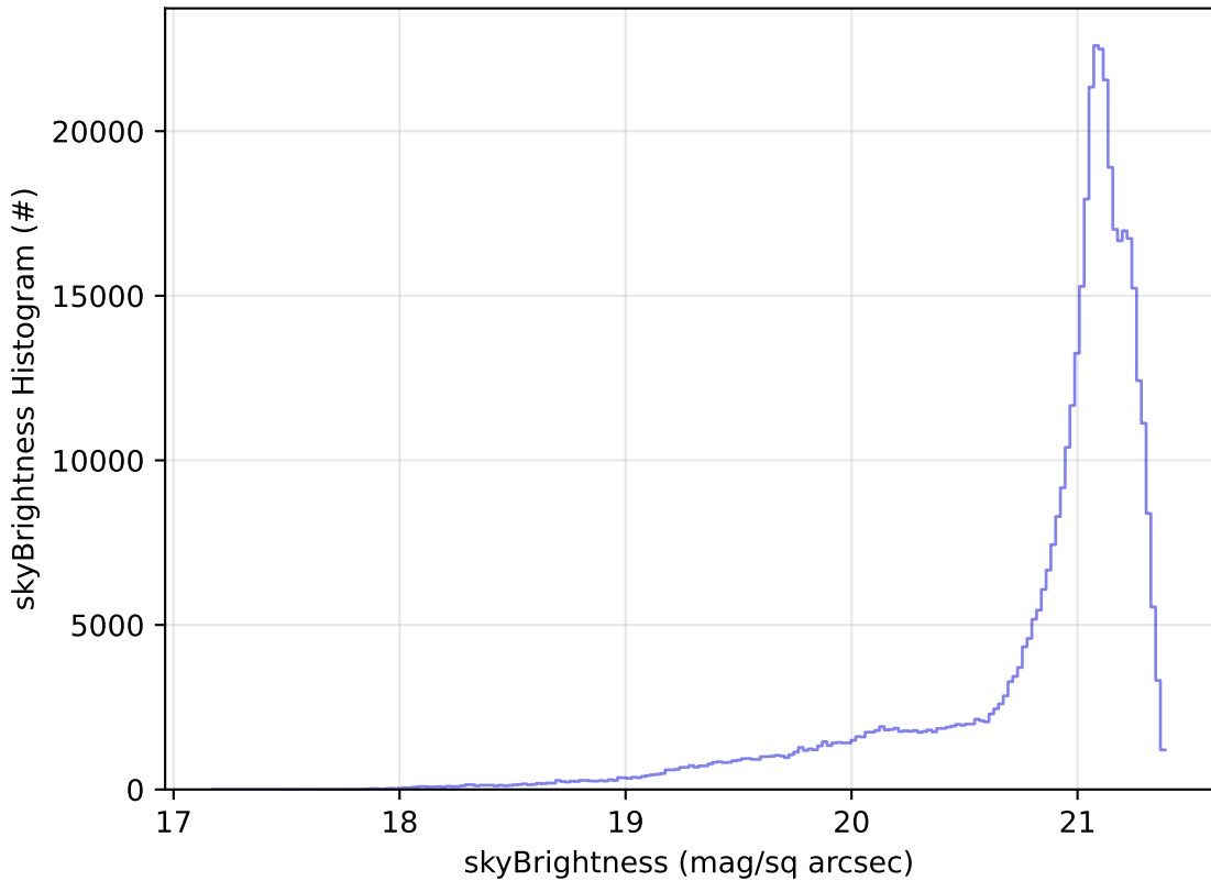
too_combined_s0.5_v3.4_10yrs All sky r band: skyBrightness Histogram
